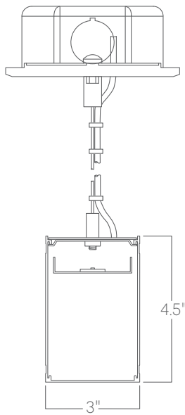
Aircraft cable
