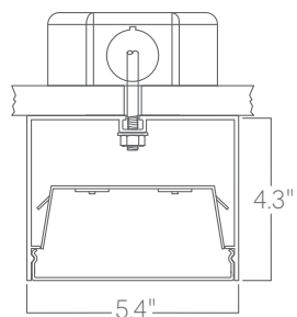
Surface mount
